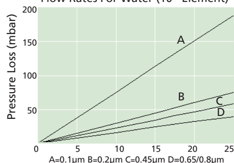
Flow Rates For Water (10" Element)
